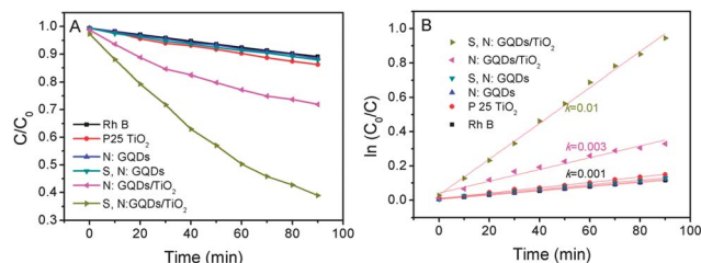
Fig. 4 Photocatalytic performance of \text{TiO}_2 , N:GQD/ \text{TiO}_2 , and S, N:GQD/ \text{TiO}_2 under visible light ( \lambda > 400 nm, A and B).
