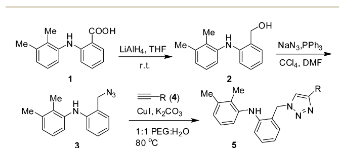
Scheme 1 Synthesis of 1,2,3-triazoles derived from mefenamic acid via a greener CuAAC approach.
