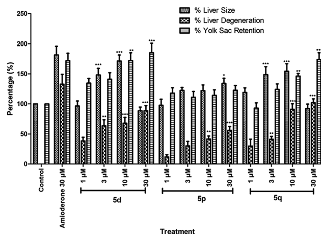
Fig. 6 Hepatotoxicity assay: the graph represents the qualitative data of percentage liver size, percentage liver degeneration & percentage yolk sac retention of three compounds at different concentrations compared to the positive control amiodarone.
