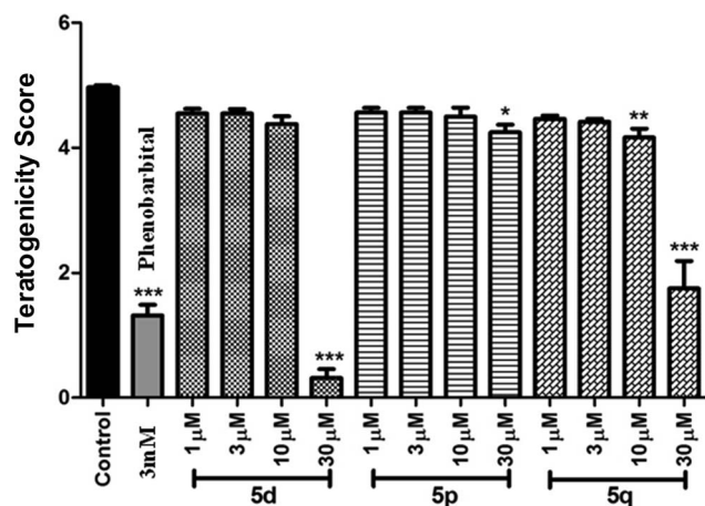
Fig. 4 Teratogenicity assay: each embryo was scored based on their level of toxicity from 5, being non toxic, to 0.5, being highly toxic. The graph represents the teratogenic scoring compared to the positive control phenobarbital.
