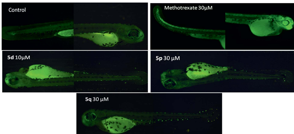
Fig. 3 Representative images of the embryos treated with compounds assayed for apoptosis.
