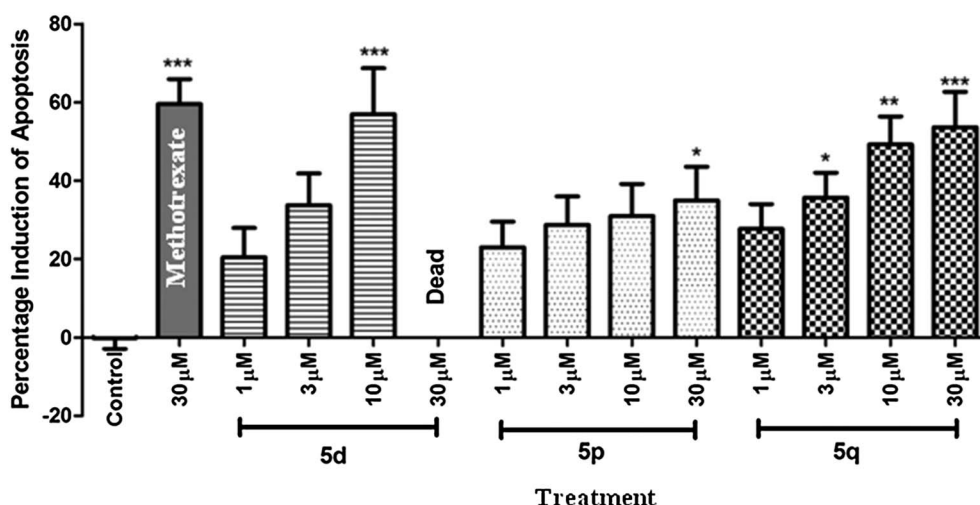
Fig. 2 The percentage induction of apoptosis caused by compounds 5d , 5p and 5q at different concentrations along with methotrexate. All the statistical analysis was performed using GraphPad Prism® software.
