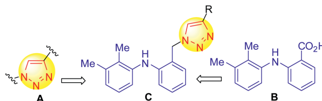
Fig. 1 The design of the new template C based on 1,2,3-triazoles ( A ) and mefenamic acid ( B ).
