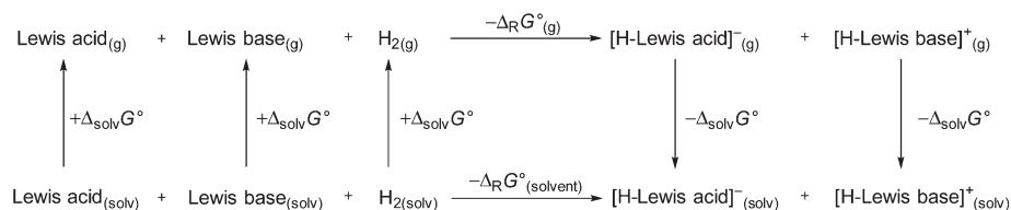
Fig. 2 Born-Haber-Fajans cycle to access the \Delta_r G^\circ_{(g)} and \Delta_r G^\circ_{(solv)} of 1 and B(C 6 F 5 ) 3 in various solvents.
