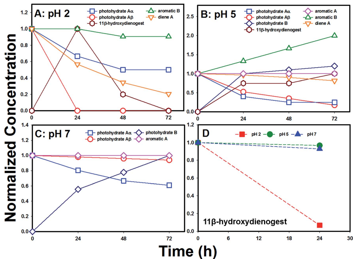
Fig. 6 Dark (thermal) stability of photoproduct mixtures at (A) pH 2, (B) pH 5, and (C) pH 7. Data in (D) show 24 h stability of isolated 11β-hydroxydienogest at pH 2, 5, and 7 (dashed lines are provided simply to help illustrate the observed trends).
