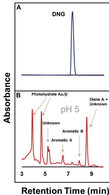
Fig. 2 LC-DAD trace of (A) DNG standard ( \lambda_{\text{det}} 310 nm) and (B) a photoproduct mixture generated at pH 5 after irradiation of DNG for 2 h ( \lambda_{\text{det}} 210 nm).
