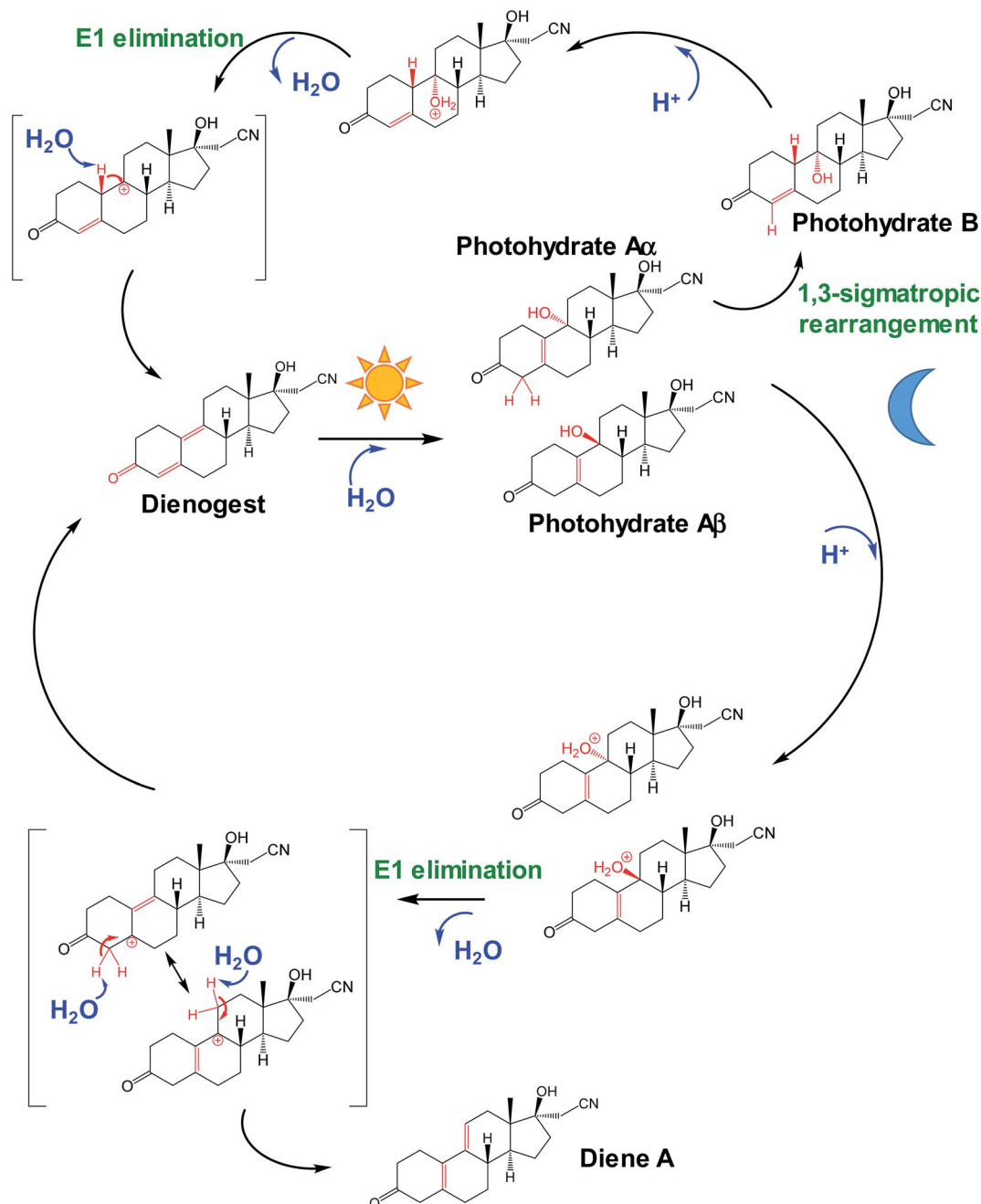
Fig. 7 Proposed reaction schematic for DNG direct photolysis and subsequent photoproduct transformations. DNG undergoes rapid photohydration yielding primary photohydrates A \alpha and A \beta . In the dark, photohydrate A \alpha can undergo a 1,3-sigmatropic rearrangement to produce secondary photohydrate B, or both primary photohydrates (A \alpha /A \beta ) can proceed through an acid-catalyzed E1 elimination resulting in either regeneration of parent DNG or formation of diene A via a resonance-stabilized carbocation intermediate. In addition, photohydrate B can proceed through an acid-catalyzed E1 elimination also resulting in regeneration of DNG.
