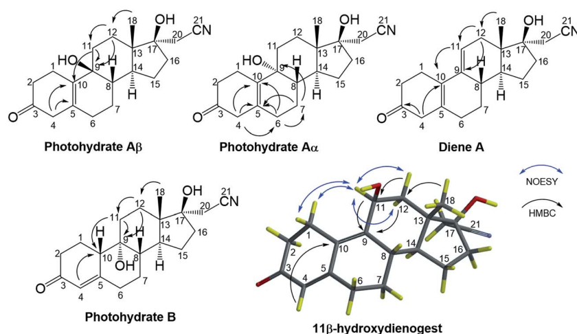
Fig. 5 Key HMBC correlations observed for three of the primary products (top): photohydrates A \alpha / \beta and diene A; and for the two isolated secondary transformation products (bottom): photohydrate B and 11 \beta -hydroxydienogest. Key NOESY correlations also shown for 11 \beta -hydroxydienogest.
