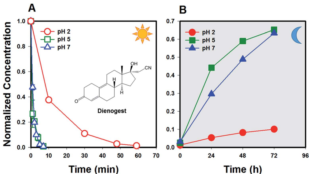
Fig. 1 Concentration of DNG ( 20 \mu\text{M} or \sim 6 \text{ mg L}^{-1} ) over time during (A) irradiation with simulated sunlight in direct photolysis experiments and (B) subsequent storage of photoproduct mixtures in the dark. Error bars represent one standard deviation from n = 3 replicates. If error bars are not visible, they are smaller than the symbol.
