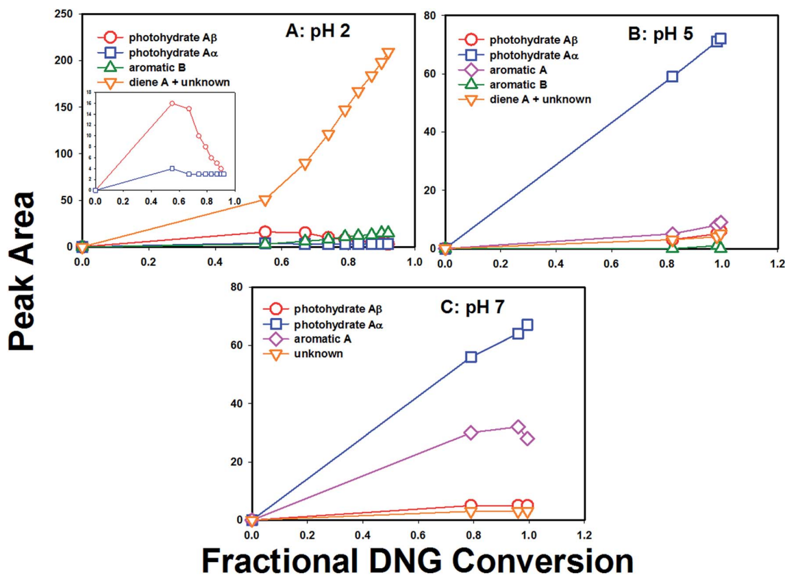
Fig. 3 Product distribution as a function of fractional DNG conversion during photolysis at (A) pH 2, (B) pH 5, and (C) pH 7, where the inset in panel A is a close-up of photohydrate A \beta and A \alpha formation at pH 2. While diene A and an as-yet unidentified compound co-eluted under the method used to collect these data (and hence they are shown as a combined peak area), the ratio of this unknown to diene A was approximately 1-to-8 at pH 2 and 1-to-1 at pH 5 based on yields from isolated product masses. Diene A was not observed at pH 7.
