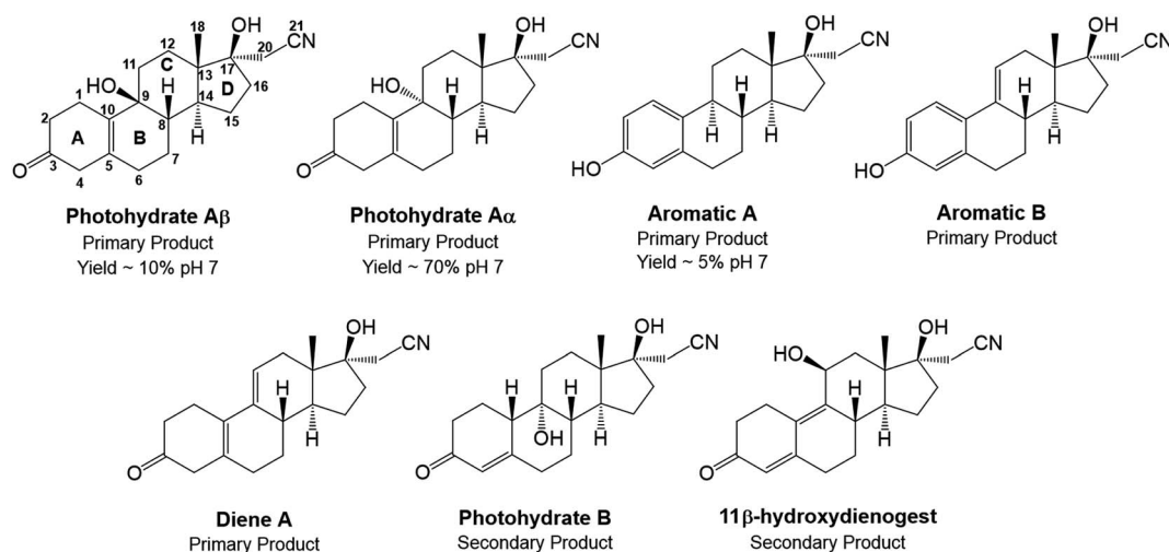
Fig. 4 Summary of primary and secondary transformation products identified during the direct photolysis of DNG across the range of pH values considered. Also provided are the yields for major products identified and quantified at pH 7.
