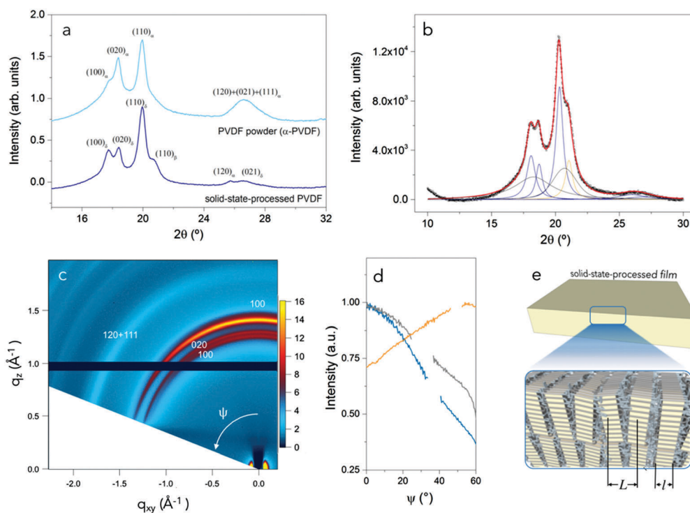
Fig. 4 X-ray diffraction data of solid-state-processed PVDF films. (a) WAXS \theta - 2\theta scans of solid-state-processed PVDF (dark blue line) and commercially bought PVDF powder (i.e., \alpha -PVDF; light blue line). (b) Decomposition of the WAXS \theta - 2\theta scans into elementary peaks of the \delta -, \alpha -, and \beta -phases. Relevant diffractions of the \delta - and \alpha -phases are plotted in blue, those of the \beta -phase are shown in orange and contribution of the amorphous halo in grey. The broad peaks correspond to the contribution of the amorphous halo. (c) 2D-WAXS pattern of solid-state processed PVDF films ( z corresponds to the direction normal to the film x - y plane). (d) WAXS intensity of the (110) reflection (blue line), ((100) + (020)) reflections (orange line) and ((120) + (021)) reflections (grey line) plotted against the \psi -angle, which is the angle defined by the rotation of the sample around an axis contained in the plane of the film ( x - y plane). (e) Schematic illustration of the preferential crystal orientation that we deduce from our X-ray data presented in (a) and (b) for solid-state-processed films.
