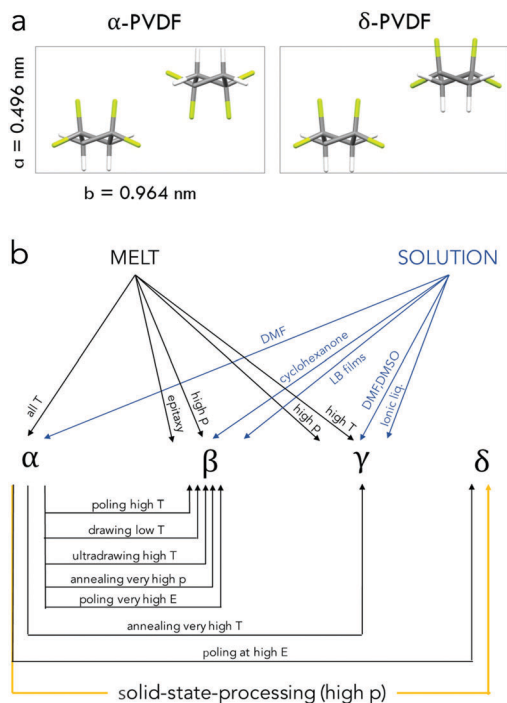
Fig. 1 Molecular arrangement and processing routes towards polar PVDF phases (adapted from ref. 9). (a) Projections onto the a - b plane of the unit cell of the chain arrangement in, respectively, \alpha - and \delta -PVDF. (b) Processing routes of PVDF towards polar forms. \delta -PVDF has been hitherto realized by applying high electric fields ( \geq 170 MV m ^{-1} ) on \alpha -PVDF, which frequently results in the breakdown of both the electrode and the polymer. Solid-state processing provides a simple, cost-efficient route to produce \delta -PVDF films.
