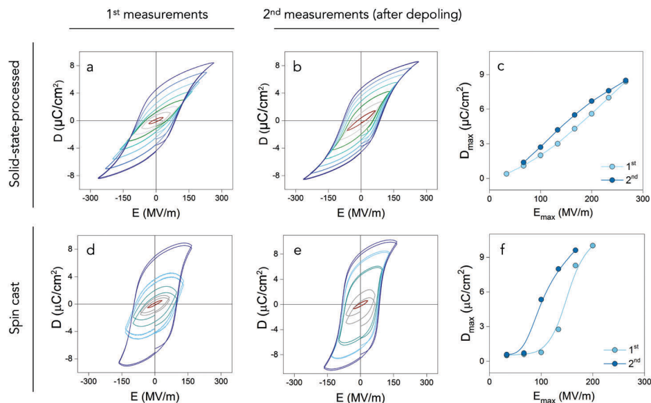
Fig. 2 Ferroelectric behaviour and piezoelectric strain of solid-state pressed and spin-cast PVDF films. (a) Hysteresis loops of solid-state processed PVDF films measured with a stepwise increasing electric field (amplitude). (b) Re-measured hysteresis loops after electrically depoling the film in (a). (c) Maximum displacement as a function of electric field for a solid-state processed PVDF film as obtained from the first and second sets of measurements. (d) Hysteresis loops of a spin-coated PVDF film measured with a stepwise increasing electric field (amplitude), which shows that the initially prepared film is electroformed into a polar PVDF at high electric field. (e) Re-measured hysteresis loops after electroforming the spin-cast PVDF film. (f) Maximum displacement as a function of electric field for a spin-coated PVDF film as obtained from the first and second sets of measurements.
