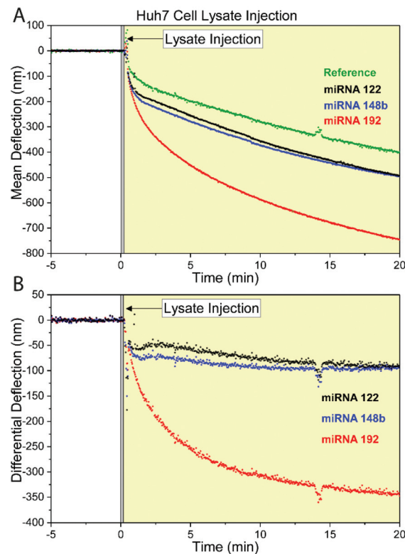
Fig. 3 Huh7 cell lysate injection. A: Mean deflection of two cantilevers per probe group (see Materials and methods). At 14 minutes there is a deviation in the reference sensor data due to cell lysate particles scattering the laser of the optical read out system. This artefact carries into the differential signal. The grey area represents an injection of 38 \mu\text{l} of diluted cell lysate at 150 \mu\text{l min}^{-1} . The yellow area indicates the incubation time after the injection, liquids stop moving and the sample interacts with the nanomechanical sensor array. Fluidic events are identical between both plots in this figure. B: Differential deflection obtained by subtracting the reference response from each of the miRNA probe responses, revealing the mechanical signal rising from the specific interaction between miRNA and the sensor bilayer. The strongest hybridisation signal is produced by the miR-192 probe. While the probes corresponding to miR-122 and 148b exhibit a diminished annealing signal. The reference probe, originating from the firefly luciferase gene, displays the smallest response. These findings match the reported RT-PCR miRNA expression studies in hepatocellular carcinoma. 21–23 Providing that the differential signal is surpassing the signal-to-noise level silicon underside passivation is not required for cantilever biological ligand detection. 37
