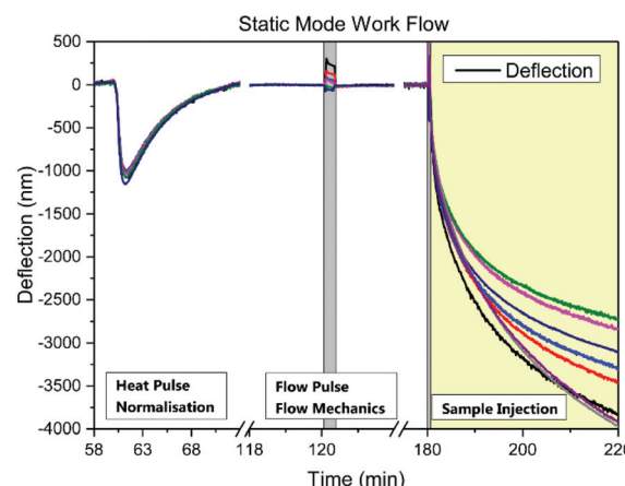
Fig. 5 Automated workflow of cantilever experiments. First, a temperature pulse (+2 °C) is induced at 60 minutes for 12 seconds to allow for subsequent mechanical normalisation between cantilevers in one array. The cantilevers bend depending on their individual bimetallic coating, a narrow distribution indicates mechanical conformity. Then, a flow pulse (38 \mu\text{L} at 150 \mu\text{L min}^{-1} ) at 120 minutes as a control experiment reveals any flow induced motion. Laminar streaming causes the cantilevers deflection. The sensors should immediately come back to the base line after the flow pulse if the flow is not altering the mechanics of the sensor. Then 38 \mu\text{L} at 150 \mu\text{L min}^{-1} of miRNA containing samples are injected and the raw data of the sensors are recorded while the solution in the fluid chamber is again stopped (yellow background). White background indicates no flow, grey areas depict buffer flow and the yellow background illustrates sample incubation.
