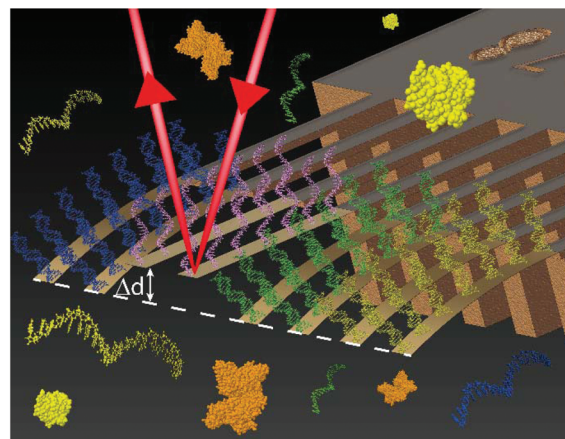
Fig. 1 Illustration of target binding on the cantilever array surface. Perspective is from inside the fluidic chamber. The laser from the optical beam read out detection method is shown reflecting away from a cantilevers surface, out of the chamber and towards the detector. Differential deflection ( \Delta d ) arise between the in situ reference probes (pink) and target sensitive probes (blue, green and yellow), four times two sensors each. Targets are captured via specific nucleic acid hybridisation on the densely packed oligonucleotide receptor layer on the top side of the sensor array. Steric hindrance of the hybridised targets on the higher populated probe sensors build-up of stress and cause a downward bending. Low concentration of proteins, globulin (yellow) and albumin (orange), are also depicted to indicate measurements in serum or plasma. The dimensions of the objects shown is not drawn to scale.
