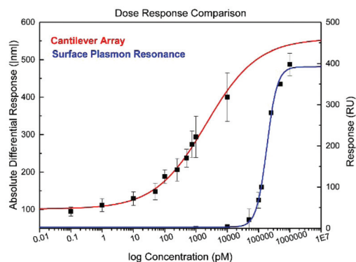
Fig. 2 Dose response comparison cantilever array versus SPR. Summarised SPR hybridisation data obtained using Biacore sensor chip functionalised with 1 \mu\text{M} thiolated probe for 1 hour. A logistic model was applied and a sigmoidal fit plotted. SPR measurements had to be conducted in pure nucleic acids spike in solutions as measurements in cell lysate were not possible due to a complete masking of the miRNA concentration signals by the lysate proteins. Error bars include chip to chip variabilities and intra chip results. Cantilever array annealing data obtained from ten miRNA target spike-in concentration experiments in Me15 cell lysate background in flow-through conditions (see Methods). Error bars are calculated using the standard deviation from three measurements. As observed the dynamic range of the cantilever based technology is larger than the one from the surface plasmon technology.
