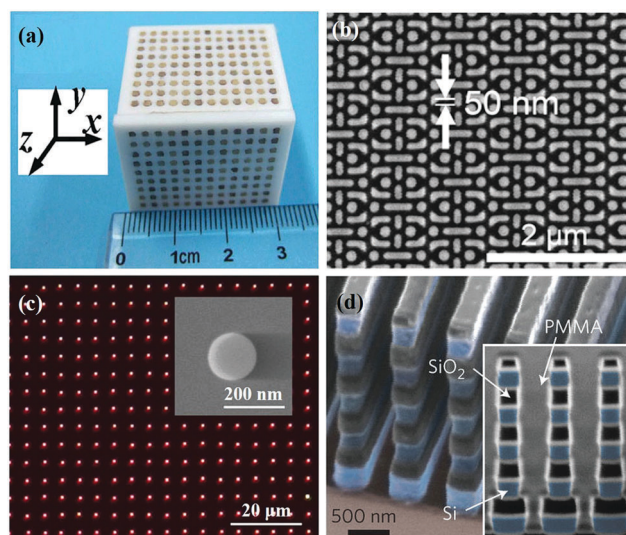
Fig. 5 Dielectric metamaterials with different structural units. (a–d) are \text{Ba}_{0.5}\text{Sr}_{0.5}\text{TiO}_3 , 58 \text{TiO}_2 , 90 silicon 91 and \text{Si}/\text{SiO}_2 dielectric metamaterials, 92 respectively. Redrawn from ref. 90. Reproduced with permission from ref. 58, 91 and 92. Copyright (2008) American Physical Society, (2014) Springer Nature and (2013) Springer Nature.
