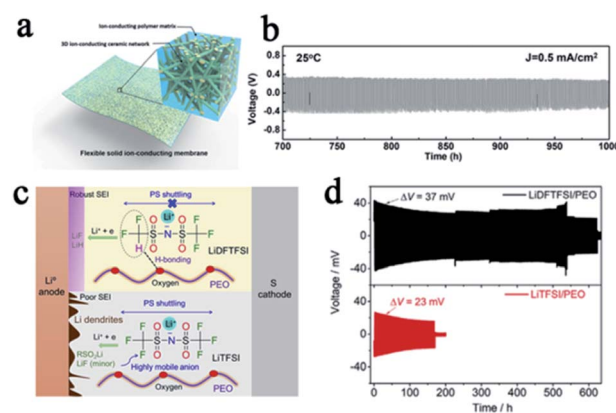
Fig. 3 (a) A schematic of the hybrid solid-state composite electrolyte and (b) the voltage profile of the continued lithium plating/stripping cycling with a current density of 0.5 mA cm -2 at 25 °C, adapted with permission from ref. 23, Proc. Natl. Acad. Sci. U. S. A. , American Institute of Physics, Copyright 2016. (c) The role of LiDFTFSI and LiTFSI in PEO and (d) the performance comparison of lithium symmetrical batteries with different SPEs, adapted with permission from ref. 32, Elsevier, Copyright 2019.
