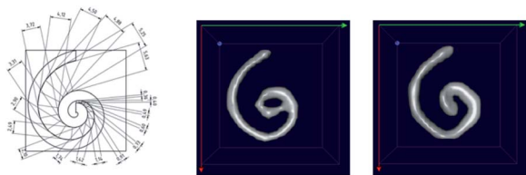
Fig. 7 Spiral phantom geometry (left) and MPI images of the phantom filled with 200 \mu\text{L} volume 15 mM iron concentration of T2 (30 nm) (right) and Resovist® (middle). The channel width of the phantom was 2 mm.
