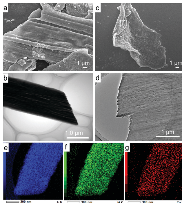
Fig. 2 Morphologies and elemental composition of the as-synthesized materials. (a) SEM image and (b) TEM image for Por-GDY . (c) SEM image and (d) TEM image for CoPor-GDY . (e) The EDS elemental mapping of CoPor-GDY .
