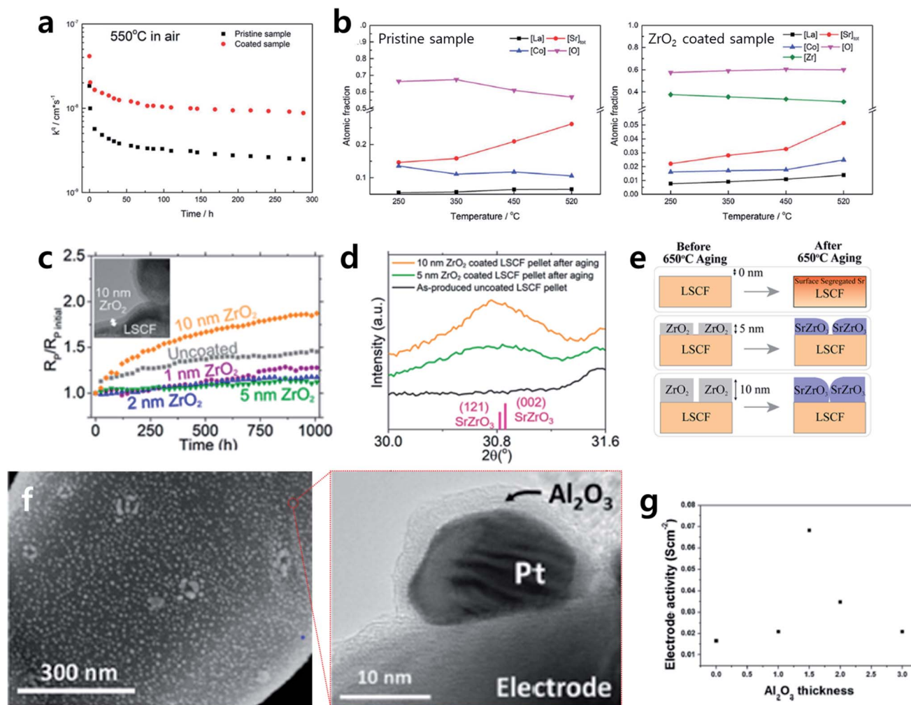
Fig. 7 (a) Time evolution of surface oxygen exchange coefficient of La 0.6 Sr 0.4 CoO 3 film electrode with and without ZrO 2 ALD coating. (b) Temperature dependent atomic concentrations of pristine and ZrO 2 coated La 0.6 Sr 0.4 CoO 3 electrode. (c) Aging behavior of normalized polarization resistance depending on the thickness of ZrO 2 ALD coating. (d) X-ray diffraction patterns obtained from pristine La 0.6 Sr 0.4 Co 0.8 Fe 0.2 O 3 , 5 nm ZrO 2 coated La 0.6 Sr 0.4 Co 0.8 Fe 0.2 O 3 , and 10 nm ZrO 2 coated La 0.6 Sr 0.4 Co 0.8 Fe 0.2 O 3 pellets after aging. (e) Schematics of proposed degradation mechanisms for uncoated and ZrO 2 coated La 0.6 Sr 0.4 Co 0.8 Fe 0.2 O 3 . (f) SEM image of Pt nanocatalysts decorated La 0.75 Sr 0.25 Cr 0.5 -Mn 0.5 O 3 electrode and TEM image of encapsulated Pt nanocatalysts by Al 2 O 3 . (g) Electrode activity for CH 4 fuel oxidation of La 0.75 Sr 0.25 Cr 0.5 -Mn 0.5 O 3 according to the thickness of Al 2 O 3 coating. Figures reproduced with permission from ref. 30, 61, and 62. Copyright 2018, The Royal Society of Chemistry, and Copyright 2020, American Chemical Society.
