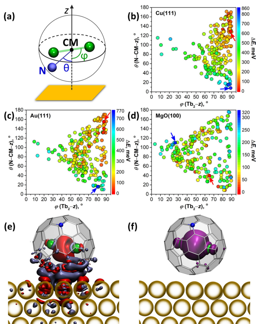
Fig. 5 (a) Definition of the \phi(\text{Tb}_2\text{-}z) and \theta(\text{N-CM-}z) angles for an adsorbed \text{Tb}_2\text{@C}_{79}\text{N} molecule, CM is the center of mass, z is the normal to the surface, Tb atoms are shown as green spheres; (b–d) distribution of \phi and \theta angles in DFT optimized structures of \text{Tb}_2\text{@C}_{79}\text{N} molecules adsorbed on Cu(111) (b), Au(111) (c), and MgO(100) (d) with their color-coded relative energies. Red and blue arrows point to the most and least stable structures, respectively. (e) Difference of the electron density for the \text{Tb}_2\text{@C}_{79}\text{N} molecule adsorbed on Au(111) (blue and red isosurfaces mark areas with decrease and increase of the electron density, respectively). (f) Spin density distribution for the structure plotted in (e).
