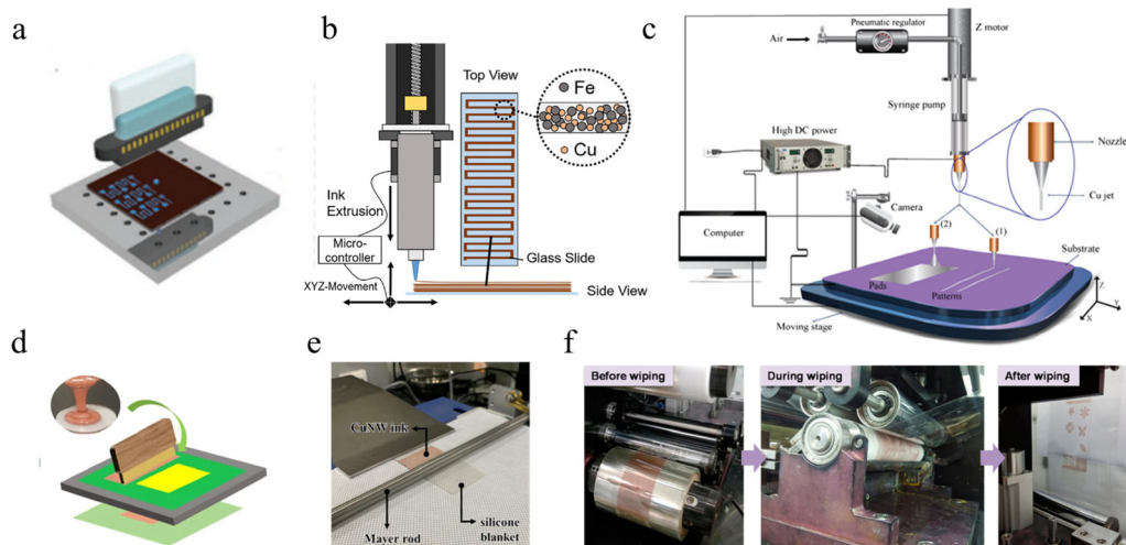
Fig. 6 Printing methods for Cu inks. (a) Schematic of inkjet printing for CuNPs. 209 Reproduced with permission from ref. 209. Copyright 2019 John Wiley and Sons. (b) Schematic of the fabrication of Cu–Fe mixed ink by direct writing. 211 Reproduced with permission from ref. 211. Copyright 2020 Elsevier. (c) Schematic diagram showing EHD jet printing. 117 Reproduced with permission from ref. 117. Copyright 2019 John Wiley and Sons. (d) Schematic illustration of screen printing. 112 Reproduced with permission from ref. 112. Copyright 2022 Springer. (e) Optical image of Mayer rod for printing CuNWs ink. 151 Reproduced with permission from ref. 151. Copyright 2022 American Chemical Society. (f) Optical image of large-scale R2R printing. 212 Reproduced with permission from ref. 212. Copyright 2016 American Chemical Society.
