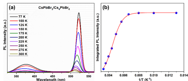
Fig. 7 (a) Temperature-dependent photoluminescence spectra of dual-phase CsPbBr 3 /Cs 4 PbBr 6 MCs measured in the temperature range of 77–300 K under \lambda_{\text{exci}} = 315 nm, and (b) integrated photoluminescence intensity of the green peak as a function of temperature.
