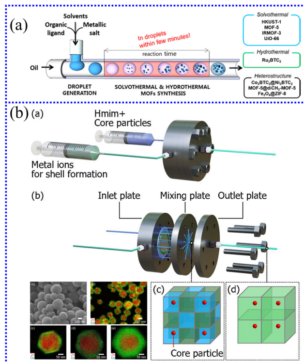
Fig. 16 (a) Homogeneous MOFs and core-shell MOFs synthesized using the microfluidic strategy. 249 Copyright 2013, American Chemical Society. (b) Zeolite imidazolate frameworks-8 (ZIF-8)@ZIF-67 and ZIF-67@ZIF-8 core-shell particles synthesized using microreactor. 251 Copyright 2021, American Chemical Society.
