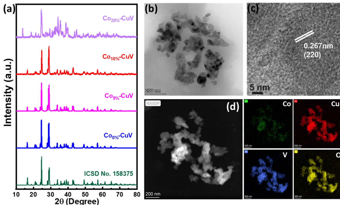
Fig. 1 (a) Powder XRD patterns of CuV and \text{Co}_x\text{-CuV} ; (b) TEM image of \text{Co}_{10\%}\text{-CuV} ; (c) HR-TEM image of \text{Co}_{10\%}\text{-CuV} ; (d) HAADF image and elemental mapping of \text{Co}_{10\%}\text{-CuV} obtained at 550 °C under an inert atmosphere.
