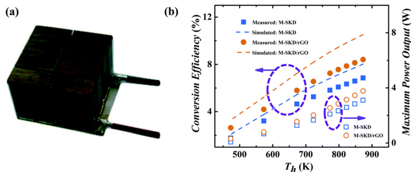
Fig. 7 A thermoelectric module (dimension of 20 mm \times 20 mm \times 16 mm) designed using \text{Ce}_{0.85}\text{Fe}_3\text{CoSb}_{12}/1.4 vol% rGO and \text{Yb}_{0.27}\text{Co}_4\text{Sb}_{12}/0.72 vol% rGO composite as p and n-type thermoelectric legs, respectively, and its (b) conversion efficiency and power outputs as a function of hot side temperature ( T_h ) for the skutterudite/rGO based devices (M-SKD/rGO) (a reference device was made from pure SKD (M-SKD)). The dash lines represent the theoretical conversion efficiency of M-SKD/rGO and M-SKD modules. Reproduced with permission from Ref. 16 Copyright 2016, Royal Society of Chemistry.
