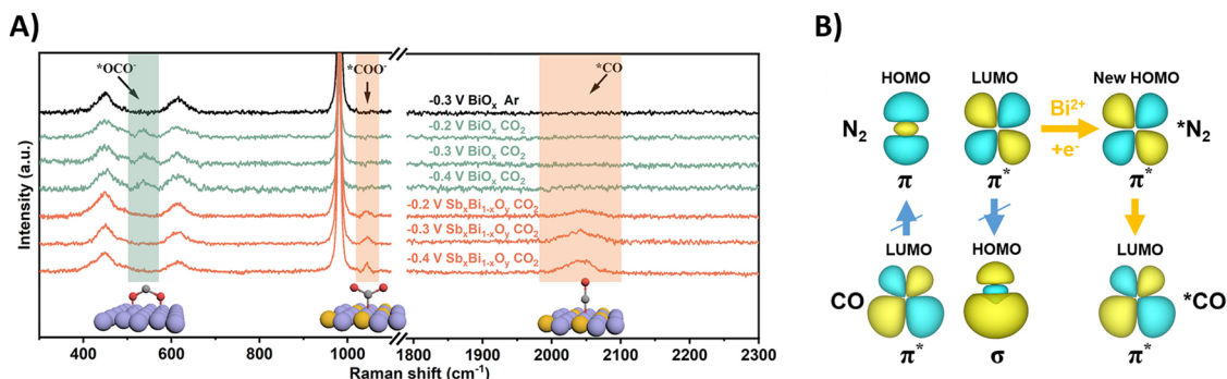
Fig. 20 Mechanistic investigations regarding CO_2 and N_2 activation using the Sb_xBi_{1-x}O_y catalyst. (A) In situ Raman spectra at different potentials. (B) The C–N coupling mechanism regulated by the symmetry matching between the HOMO of ^*N_2 and the LUMO of ^*CO . Adapted from ref. 203.
