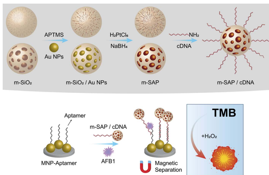
Fig. 8 Schematic presentation of nanozyme and aptamer-based immunosorbent assay (NAISA): (A) preparation of \text{m-SAP/cDNA} and (B) construction of NAISA for AFB1 detection.
