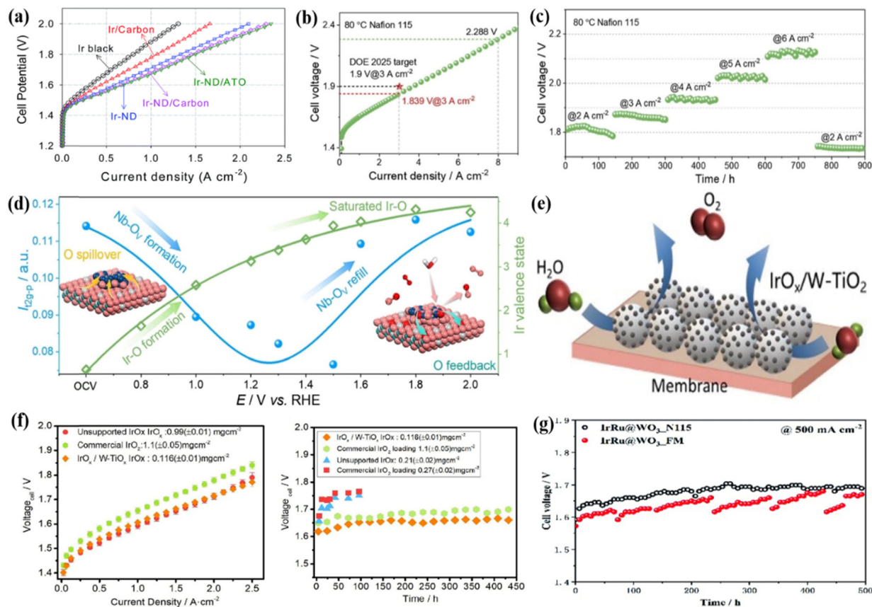
Fig. 5 (a) Single cell performance of Ir-ND catalysts with a catalyst loading of 1.0 mg cm -2 at 80 °C. Reproduced with permission from ref. 80. Copyright 2017, Elsevier B.V. (b) Polarization curve of the PEMWE device with Ir/Nb 2 O 5-x as the anode catalyst and (c) stability curves of the electrolyzer at gradient increasing current densities of 2, 3, 4, 5, and 6 A cm -2 . (d) An illustration of the dynamic interface effect and the variation of the Ir valence state of Ir/Nb 2 O 5-x . Reproduced with permission from ref. 136. Copyright 2022, Wiley-VCH GmbH. (e) An illustration of the MEA with an anode catalyst layer. (f) Polarization curves and durability test curves of the PEMWE device with different MEAs at 80 °C. Reproduced with permission from ref. 140. Copyright 2021, Elsevier Ltd. (g) The single cell voltage curves of IrRu@WO 3 during stability testing at 80 °C. Reproduced with permission from ref. 141. Copyright 2022, The Royal Society of Chemistry.
