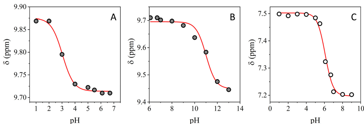
Fig. 3 (A) and (B) in gray circles, chemical shift ( \delta_{\text{obs}} ) vs. pH for the aldehyde proton (9.9 to 9.4 ppm); (C) in white circles, chemical shift ( \delta_{\text{obs}} ) vs. pH for the nitrogen proton (7.5 to 7.2 ppm). The red line represents the non-linear fitting to eqn (1).
