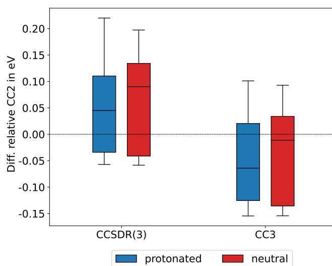
Fig. 7 Correction with CCSDR(3) and CC3 for the neutral and the protonated species of the photobases.
