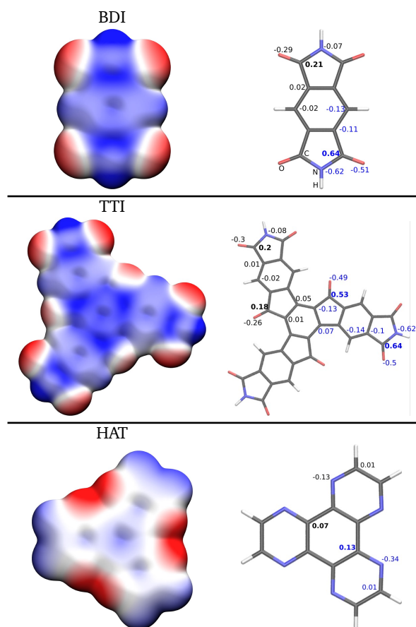
Fig. 4 Electrostatic potential maps for selected \pi systems, mapped on the electron density iso-surface of 0.001 a.u. The red color corresponds to a negative region of the electrostatic potential (-0.04 au), whereas the blue color corresponds to the region where the potential is positive (+0.04 au). Charges (NBO in blue and Hirschfeld in black) are indicated for heteroatoms.
