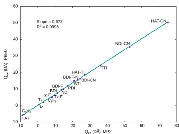
Fig. 2 Correlation curve between quadrupole moments Q_{zz} (DÅ) computed at the MP2 and PBE0-D3 levels. Labels for molecules as in Figure 1.
