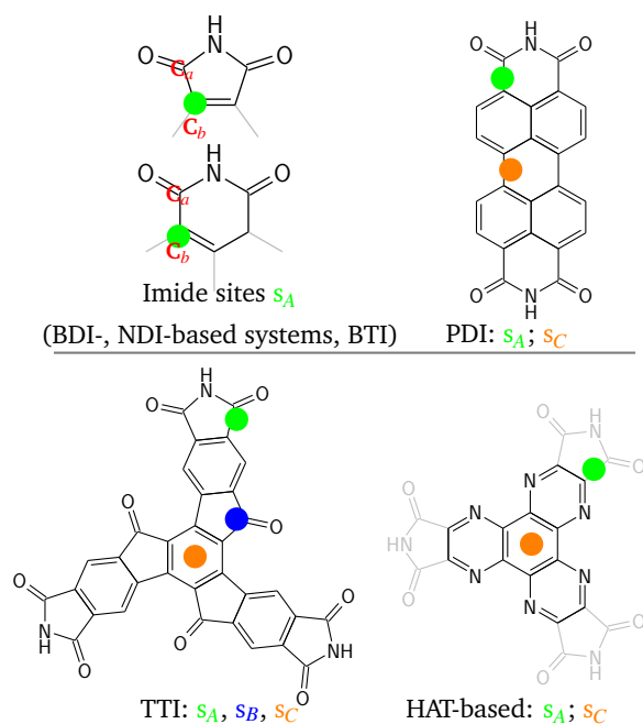
Fig. 3 Top view of the chloride binding sites. Green circles indicate positions close to the imide ( s_A ), orange circles are on the most central rings ( s_C ), and the blue circle indicates a site close to the cyclopentenone moiety ( s_B ).
