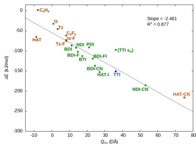
Fig. 5 Smallest MP2 computed \Delta E values (among the tested adduct structures) as a function of the Q_{zz} of each \pi system. Orange, green and blue dots refers to s_C , s_A and s_B binding sites, as in Figure 3. The value for the TTI s_A case is also reported (but not used for the regression).
