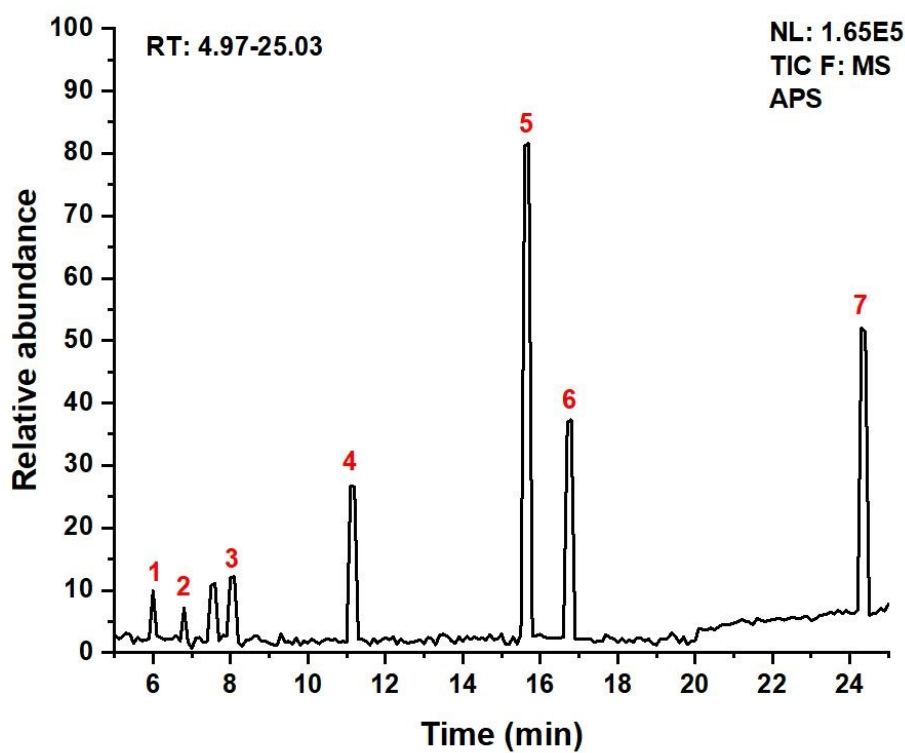
Fig. 7 GC-MS chromatogram for monosaccharide composition of polysaccharide isolated from amla pomace sweetmeat (1-xylose; 2- mannose; 3- glucose; 4- rhamnose; 5- galacturonic acid; 6- arabinose; 7- galactose)
