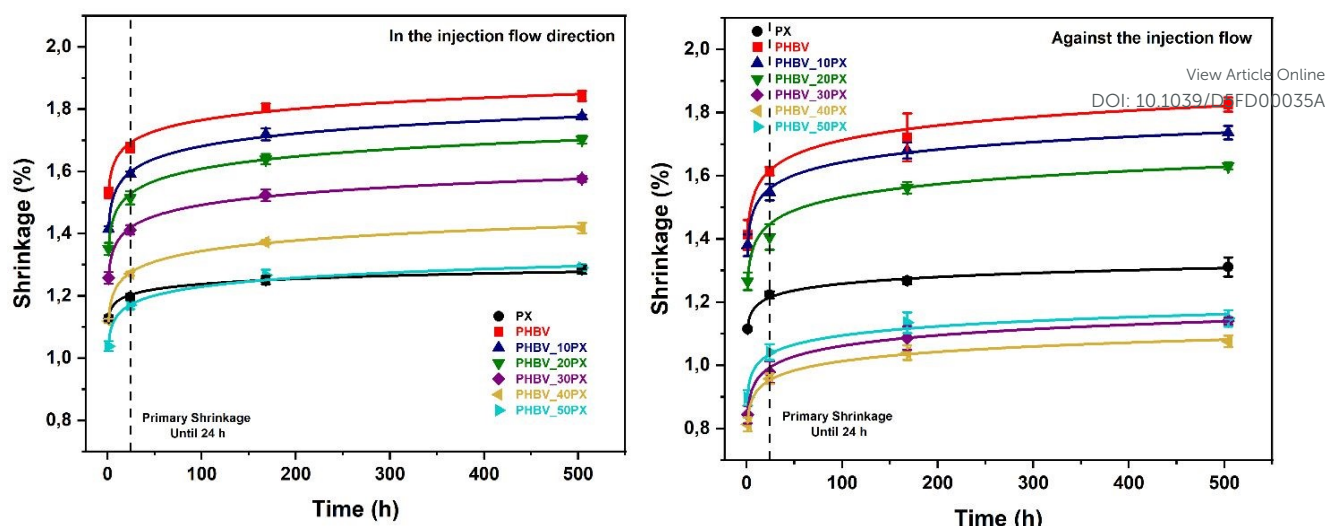
Fig 7. Shrinkage of the samples of all compositions: (a) in the direction of the injection flow; (b) in against direction of the injection flow, with 400 bar of holding pressure
