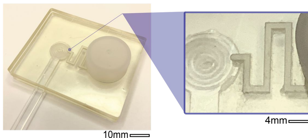
Figure 1: Design and assembly of the O2C system for automated elution of antigens. A) Exploded CAD renderings of the O2C components. The rendering on the left contains a CandyCollect which has open channels and has yet to be sealed. The rendering on the right shows the entire system when it is assembled and the microchannels on the CandyCollect are fully enclosed. B) Image of the 3D-printed O2C device with fully assembled components. The inset to the right highlights the connection between the reagent channel on the top layer of the O2C and the CandyCollect.
