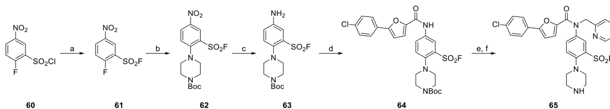
Scheme 6 Synthesis of compound 65 . Reagents and conditions: (a) \text{KHF}_2 , \text{MeCN}/\text{H}_2\text{O} (2 : 1, V/V), rt, 18 h, quant.; (b) 1-Boc-piperazine, DIPEA, DMF, 80 °C, 3 h, 54%; (c) \text{Pd}/\text{C} , \text{H}_2 , \text{MeOH} , rt, 1 h, quant.; (d) 5-(4-chlorophenyl)furan-2-carboxylic acid, HATU, DIPEA, DMF, 80 °C, 17 h, 37%; (e) 2-(bromomethyl)pyridine \text{HBr} , \text{NaH} , DMF, rt, 20 h; then (f) TFA, DCM, rt, 2 h, 42% over two steps.
