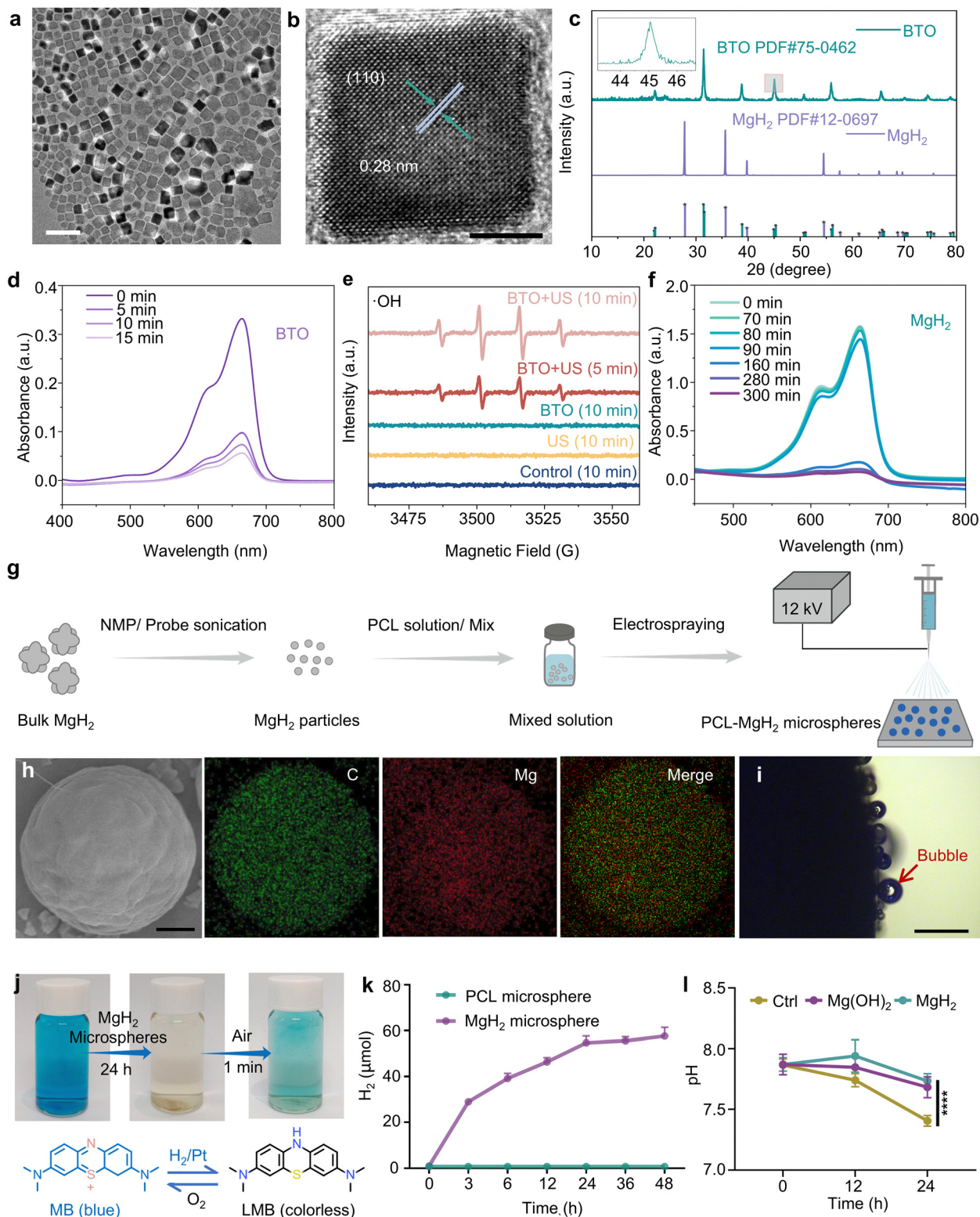
Fig. 2 Characterization of BTO nanoparticles and MgH 2 microspheres. (a) TEM image (scale bar = 50 nm) and (b) high-resolution transmission electron microscopy (HRTEM) image of BTO nanoparticles (scale bar = 5 nm). (c) XRD pattern of BTO nanoparticles (insert image of the enlarged (002 and 200) peaks) and MgH 2 particles. (d) UV-vis absorbance spectra of MB under US irradiation (1.0 MHz, 1.0 W cm -2 , 50% duty cycle) in the presence of BTO nanoparticles. (e) ESR spectra of \cdot\text{OH} trapped by DMPO under different experimental conditions. (f) UV-vis absorbance spectra of MB-Pt after reduction of MB by H 2 generated by MgH 2 at different time points. (g) Process for the preparation of PCL-MgH 2 microspheres (it was shortened to MgH 2 microspheres in the latest article). (h) SEM images and elemental mapping of MgH 2 microspheres (scale bar = 1 \mu\text{m} ). (i) Photograph of bubbles generated on the surface of a PCL tablet containing MgH 2 in it. (The bubbles on the surface of the tablet could be easily observed compared with MgH 2 microspheres, scale bar = 500 \mu\text{m} .) (j) Photograph showing reversible disappearance of the blue color of the MB-Pt probe (10 \mu\text{g mL}^{-1} MB + 60 \mu\text{g mL}^{-1} Pt) after H 2 reduction and air contact. (k) Released H 2 in 1x PBS measured by gas chromatography (GC). (l) pH value changes of the buffer in the presence of Mg(OH) 2 microspheres and MgH 2 microspheres measured by pH microelectrode.
