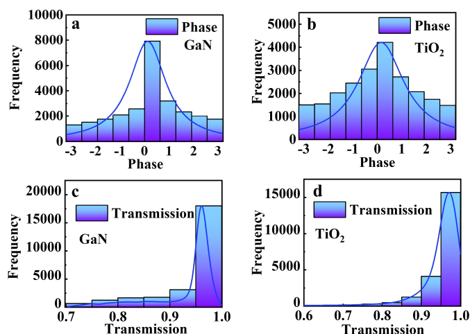
Fig. 2 (a,b) Phase and (c,d) Transmission data for GaN and TiO 2 .
