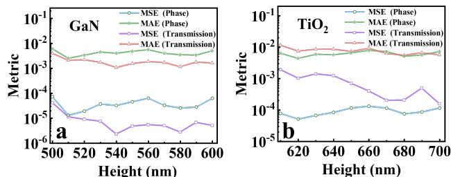
Fig. 5 Leave-One-Height-Out-Cross-Validation results for phase and transmission model for (a) GaN and (b) TiO 2 .
