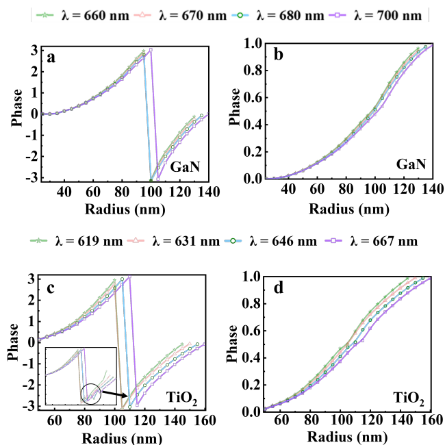
Fig. 3 Phase response (a,c) after filtering, with the inset of (c) showing damped variations. (b,d) after normalization.
