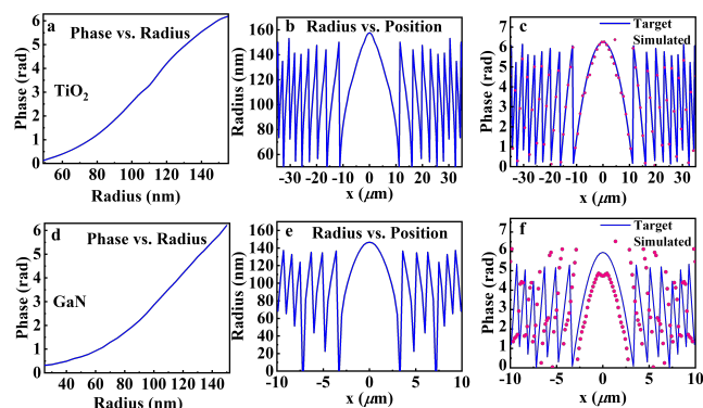
Fig. 10 Metalens design workflow: (a,d) phase vs. radius library from predicted data (b,e) Translated radius vs. position distribution (c,f) Comparison of target and simulated phase profile.
