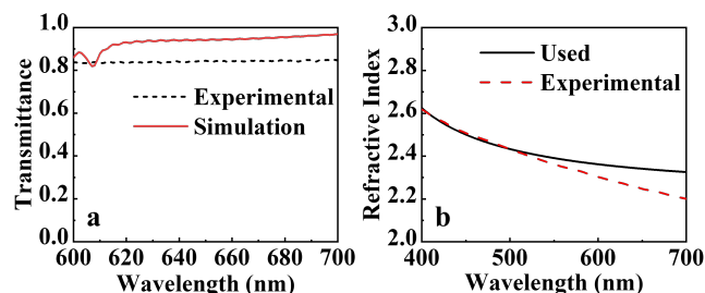
Fig. 9 (a) Experimental and simulated transmittance spectra and (b) Used and experimental refractive index of the \text{TiO}_2 thin film as a function of wavelength.
