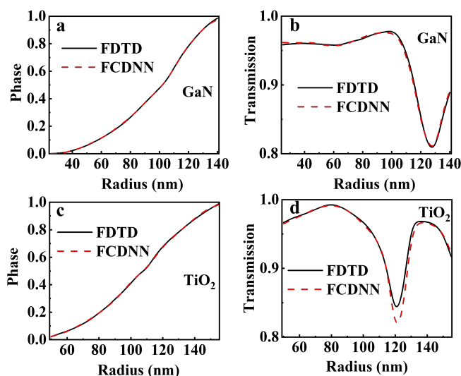
Fig. 7 Comparison between simulated (FDTD) and predicted (FCDNN) phase (a,c) and transmission (b,d) response for GaN and \text{TiO}_2 , respectively.
