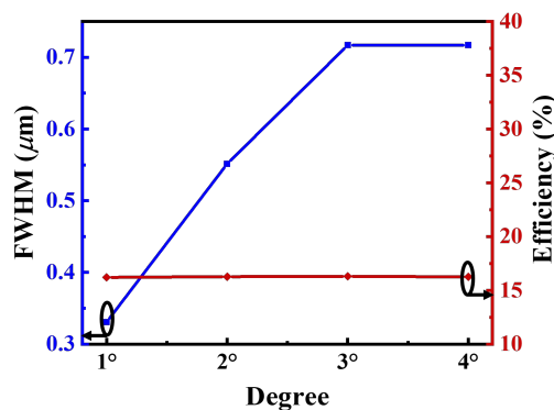
Fig. 14 FWHM and efficiency as a function of incident angle of the metalens with an aperture stop of 10\ \mu\text{m} .
