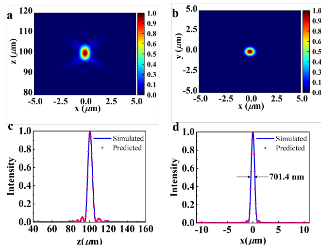
Fig. 11 Intensity profile of \text{TiO}_2 based metalens (a) in ( x - z plane) and (b) in ( x - y plane) of the focal spot in the focal plane. (c) Normalized intensity distribution (simulated and predicted) at the focal point along propagation direction ( z -axis). (d) Corresponding horizontal cut at the focal spot in (b). Here, FWHM of the focal spot is 701.4 nm.
