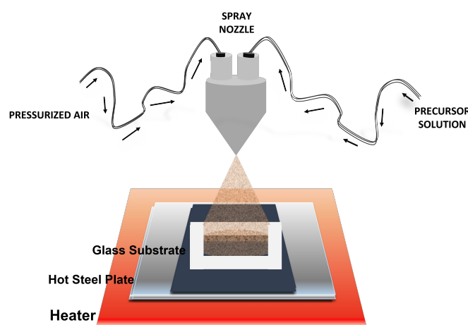
Fig. 8 Schematic diagram of \text{TiO}_2 thin film deposition using a homemade spray pyrolysis.
