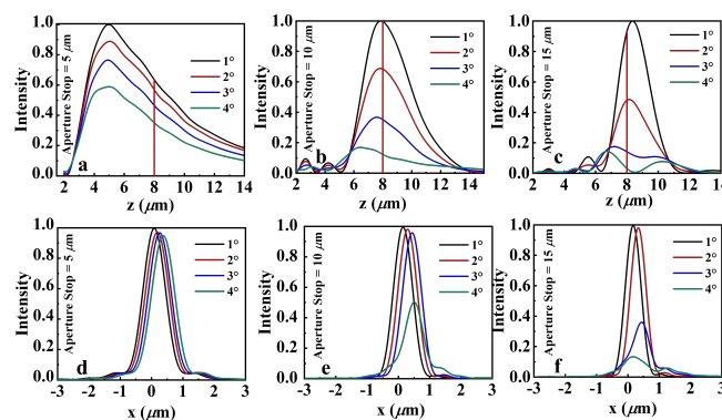
Fig. 13 Normalized intensity plots for GaN metalens along z and x -axis for aperture stop at (a,d) 5\ \mu\text{m} , (b,e) 10\ \mu\text{m} , and (c,f) for 15\ \mu\text{m} . The vertical red line indicates the focal length.
