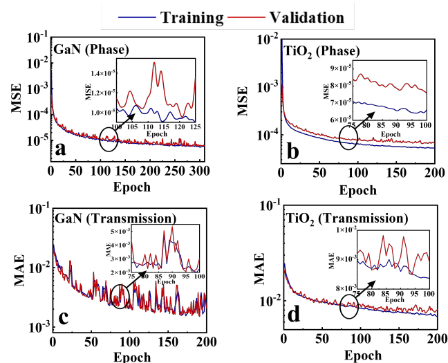
Fig. 6 Learning curves of phase (a,b) and transmission (c,d) models for GaN and TiO 2 , respectively.
