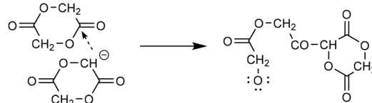
Scheme 4 Reversible deprotonation of glycolide and subsequent side reaction.
