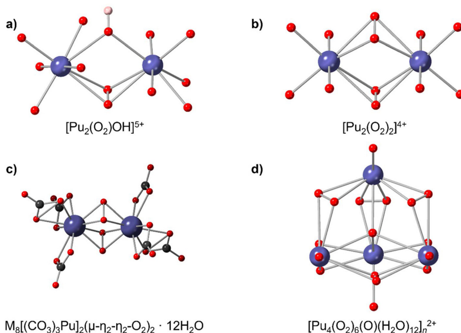
Fig. 9 \text{Pu(IV)} peroxo-complexes such as (a) [\text{Pu}_2(\text{O}_2)(\text{OH})]^{5+} , (b) [\text{Pu}_2(\text{O}_2)_2]^{4+} , (c) \text{M}_8[(\text{CO}_3)_3\text{Pu}]_2(\mu\text{-}\eta^2\text{-}\eta^2\text{-O}_2)_2\cdot 12\text{H}_2\text{O} (where \text{M} = \text{K} or \text{Na} ), and (d) [\text{Pu}_4(\text{O}_2)_6(\text{O})(\text{H}_2\text{O})_{12}]^{2+} . \text{Pu} , \text{O} , \text{C} , and \text{H} are represented as purple, red, grey, and pink spheres, respectively. Hydrogens on aqua ligands, outer sphere waters molecules, and counter cations were omitted for clarity. 95–97
