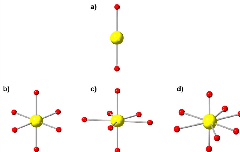
Fig. 6 Ball-and-stick models of the hexavalent and pentavalent (a) uranyl cation (UO 2 2+ /UO 2 + ) and potential geometries—(b) tetragonal, (c) pentagonal, and (d) hexagonal bipyramids—that are found in solution and solid-state materials. Adapted from Plášil. 70
