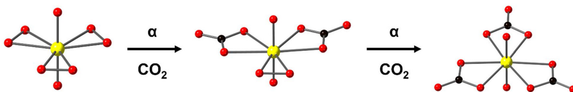
Fig. 14 Direct CO 2 capture by a uranyl triperoxide moiety upon exposure to α-radiation, resulting in the formation of a uranyl tricarbonates species. Adapted from Fairley et al. 234
