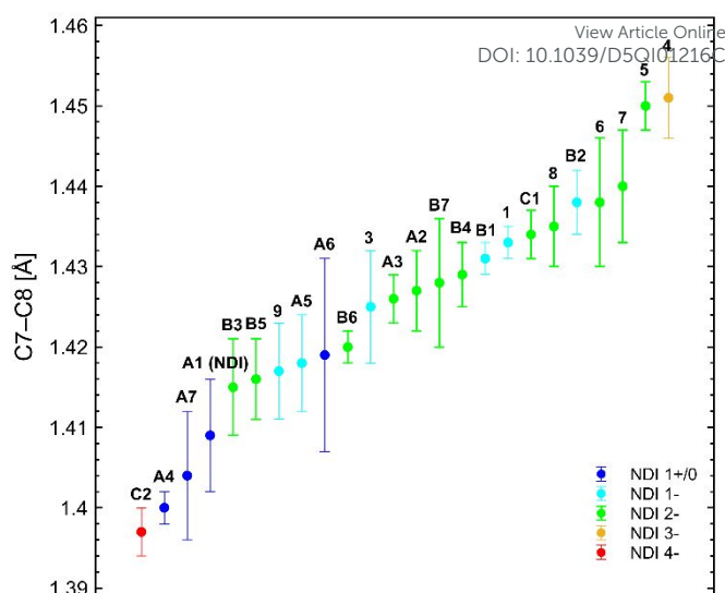
Fig. 10 Bond length of the C7–C8 bond in NDI complexes in varying formal oxidation states. Trend to differentiate between three-time ( > 1.45 Å) and four-time reduction ( < 1.40 Å) of NDI. See ESI † (Table S7) for the full set of data points.
