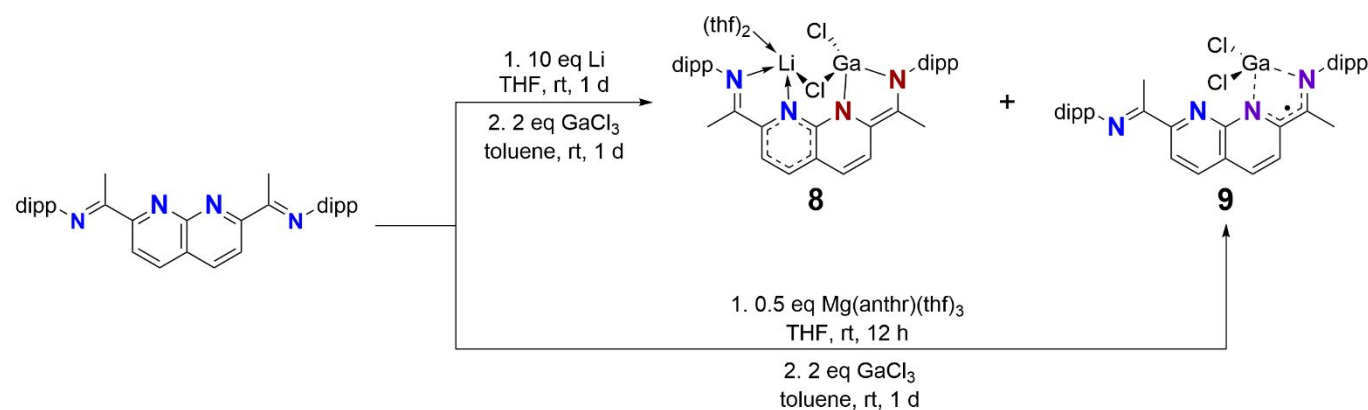
Scheme 5 Reaction of with lithium pre-reduced NDI and GaCl 3 , and an alternative route via pre-reducing with Mg(anthr)(thf) 3 .
