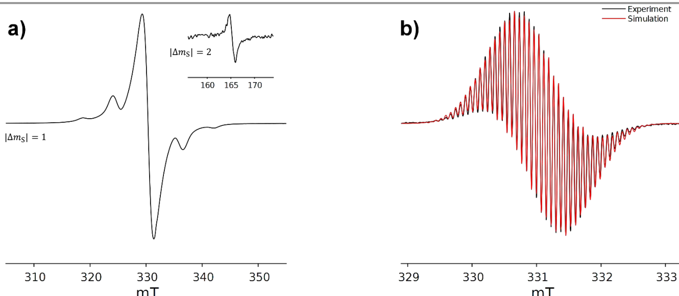
Fig. 5 (a) EPR (X-Band, \nu = 9.2564 GHz) spectrum of a frozen solution of compound 3 in THF at 123 K ( |\Delta m_S| = 1 region) with an inset of the |\Delta m_S| = 2 region. (b) Experimental EPR spectrum (X-Band, \nu = 9.2564 GHz) and simulated spectrum of a solution of compound 3 in Et 2 O at 298 K. Parameters for the simulation: S = 1 , g = 2.00715 , Gaussian line width (lwpp) = 0.05 mT, (4*) A_N = 4.23 MHz, (2*) A_{N'} = 2.12 MHz, (2*) A_{N''} = 1.07 MHz, (6*) A_H = 10.70 MHz.
