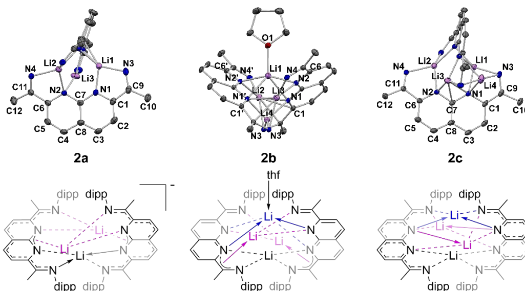
Fig. 3 Molecular structure of complexes 2a – 2c (top). All atoms are represented by atomic displacement ellipsoids set at 50% probability. Solvent molecules, hydrogen atoms, and carbon atoms of the substituents, as well as a [\text{Li}(\text{thf})_4]^+ fragment for complex 2a are omitted for clarity. (for metrics, see ESI†). Schemes corresponding to complexes 2a – 2c to visualise binding situation (bottom).
