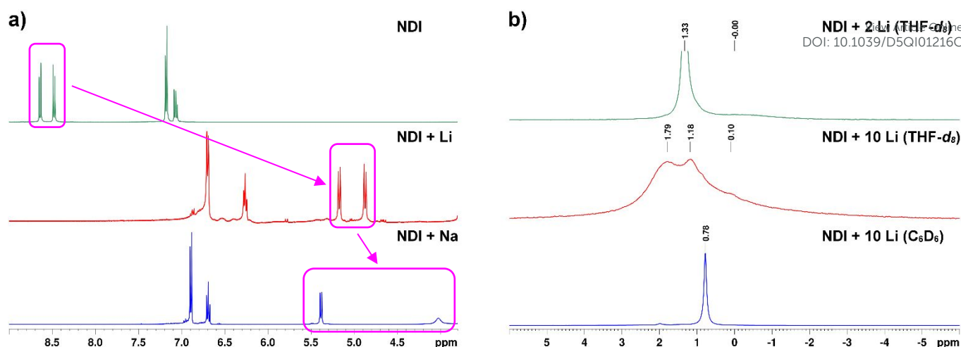
Fig. 2 (a) ^1\text{H} -NMR spectra in \text{THF-}d_8 of NDI (top), NDI with 10 equivalents of granular lithium (middle) and NDI with two equivalents of sodium metal (bottom). Marked (magenta) are the proton signals of the protons at C3 and C4. (b) ^7\text{Li} -NMR spectra of the reaction mixtures of NDI and granular lithium with two equivalents in \text{THF-}d_8 (top), with 10 equivalents in \text{THF-}d_8 (middle), and with 10 equivalents in \text{C}_6\text{D}_6 (bottom).
