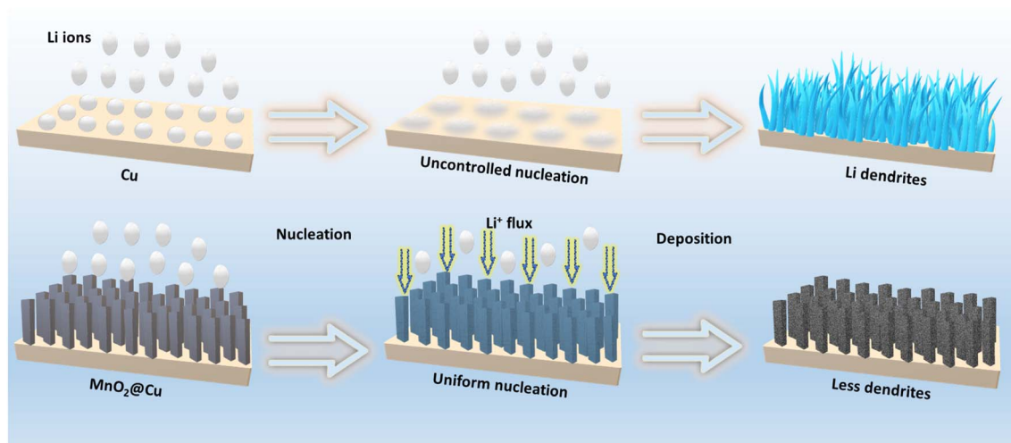
Fig. 4 Lithium growth behavior during plating on bare Cu and \text{MnO}_2 -modified Cu current collectors.
