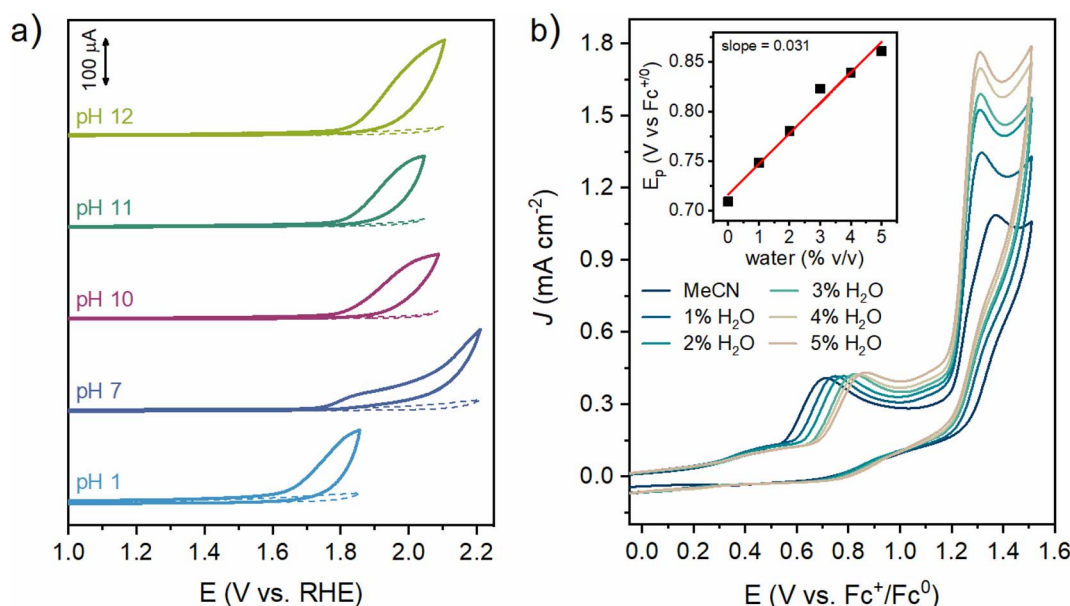
Fig. 2 (a) pH-dependent cyclic voltammograms of [\text{IrCp}^*\text{Cl}(\text{dppz})]\text{Cl} (1 mM) in aqueous solution. The dashed lines show the blank CVs in the absence of a catalyst. Conditions: glassy carbon working electrode, \text{Ag}/\text{AgCl}/\text{KCl} (3 M) reference electrode, Pt wire counter electrode, 0.1 M electrolyte, and a scan rate of 100 \text{ mV s}^{-1} . (b) Cyclic voltammograms of [\text{IrCp}^*\text{Cl}(\text{dppz})]\text{Cl} (1.0 mM) in neat MeCN and with increasing water content (1–5%). Inset shows the linear fit of the shift of the peak potential for the first oxidation step against the concentration of water. Conditions: glassy carbon working electrode, Pt wire counter electrode, \text{Ag}/\text{AgNO}_3 (10 mM) reference electrode, and \text{TBABF}_4 (0.1 M) supporting electrolyte.
