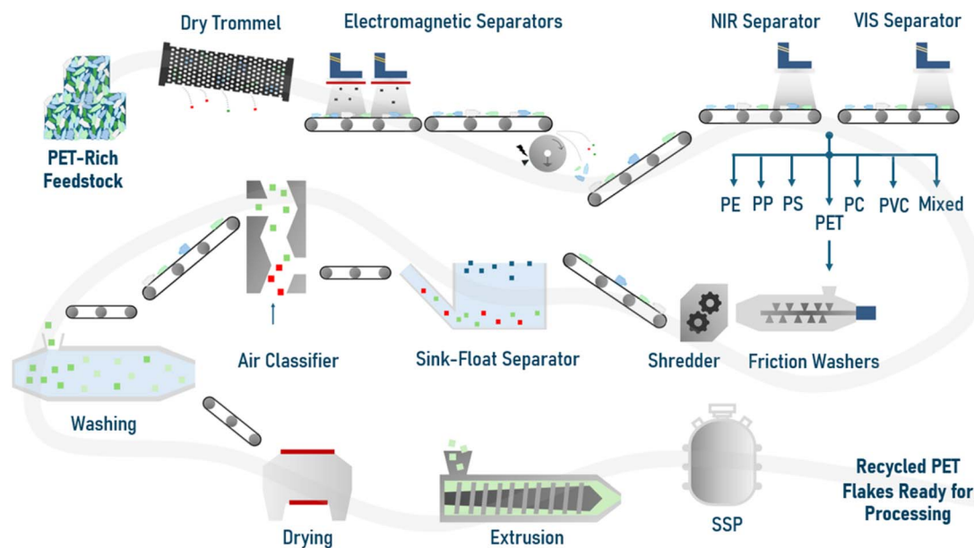
Fig. 6 Key steps of PET mechanical recycling. Steps can sometimes be omitted or altered; e.g. extrusion and solid-state modification can be in a different configuration (or order).
