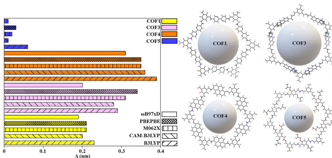
Fig. 3 (Left) Cumulative pore diameter \Delta histograms (nm) at the functional/6-311G(d,p) level in the gas phase for the studied COFs. (Right) Optimized structures at the \omega B97XD/6-311G(d,p) level.
