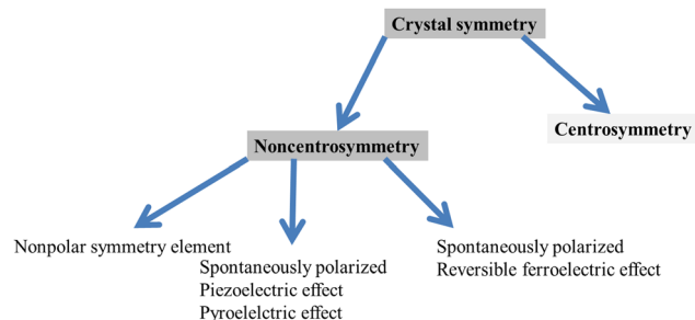
Scheme 6 Halide perovskite crystal symmetry showing ferroelectricity, piezoelectricity and pyroelectricity effects.
