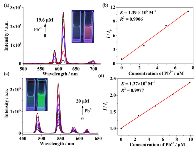
Fig. 9 Fluorescence spectra of complexes (a) 3 and (c) 5 with the increase of \text{Pb}^{2+} concentration; Stern–Volmer linear fitting of I/I_0 to \text{Pb}^{2+} ions in the low concentration range in suspensions of complexes (b) 3 and (d) 5.
