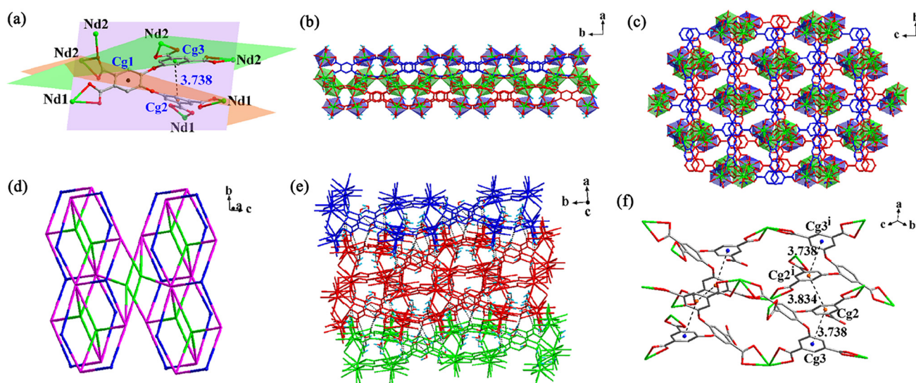
Fig. 2 (a) Coordination mode of the ligand \text{L}^{6-} in 1 (the sky blue represents H atom; the three different colored planes represent the planes of the three benzene rings in the ligand); (b) 1D chain structure; (c) 2D structure; (d) Topological structure; (e) 3D network formed by hydrogen bonds; (f) \pi\cdots\pi interactions present in complex 1.
