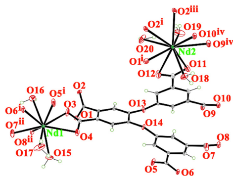
Fig. 1 Coordination environments of \text{Nd}(\text{III}) ions in complex 1, symmetry codes: (i) x, 1/2 - y, 1/2 + z ; (ii) x, -1 + y, z ; (iii) -x, 1/2 + y, 1.5 - z ; (iv) x, 1.5 - y, 1/2 + z .
