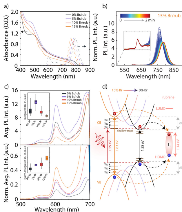
Fig. 8 (a) Absorption and normalized emission for MA 0.85 FA 0.15 Pb(Br x I 1-x ) perovskite bilayer films of varying bromide concentrations ( x = 0, 5, 10 , and 15 ). (b) Time-dependent PL measurement of the 15% bromide composition bilayer film where an observable bathochromic shift to the perovskite emission is observed. Inset magnifies the rubrene emission at 600 nm. All PL measurements were taken under 405 nm continuous wave excitation. (c) Average upconverted PL emission for the mixed halide MAFA bilayer films (top). Average upconverted PL emission of the mixed halide MAFA bilayer films normalized to the overlap integral of the film absorbance and 780 nm laser emission (bottom). Box plot insets in (c) show integrated upconverted PL intensities for the bilayer films taken across 20 spots for two sample sets. (d) Schematic illustrating the sensitization process assisted by trap-states within the perovskite for the mixed halide compositions. Adapted from ref. 114 with permission of AIP Publishing, copyright 2021.
