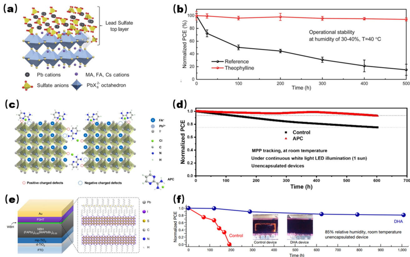
Fig. 2 (a) Schematic diagram of the protection of perovskites by in situ formation of a \text{PbSO}_4 top layer on the perovskite surface. Reproduced with permission. 61 Copyright 2019 Science. (b) Efficiency evolution measured for theophylline-treated or non-theophylline-treated packaged PSCs exposed to constant illumination ( 90 \pm 10 \text{ mW cm}^{-2} ). Reproduced with permission. 60 Copyright 2019 Science. (c) Schematic diagram of the proposed interaction mechanism between 2-amidinopyrimidine hydrochloride and the perovskite. 52 (d) Dynamic MPP tracking of the unencapsulated 2-amidinopyrimidine hydrochloride treated and control devices under constant illumination. Reproduced with permission. 52 Copyright 2022 The Royal Society of Chemistry. (e) Left, structure of the PSC based on a double-layered halide architecture using P3HT as the HTM. Right, schematic diagram of the interface between the wide bandgap halide and P3HT. 76 (f) Results of humidity stability tests on the unsealed double-layered halide device and control devices under 85% RH at RT. Inset, photographs of the double-layered halide architecture (right) and the control (left) device after 200 h under 85% RH at RT. Reproduced with permission. 76 Copyright 2019 Nature.
